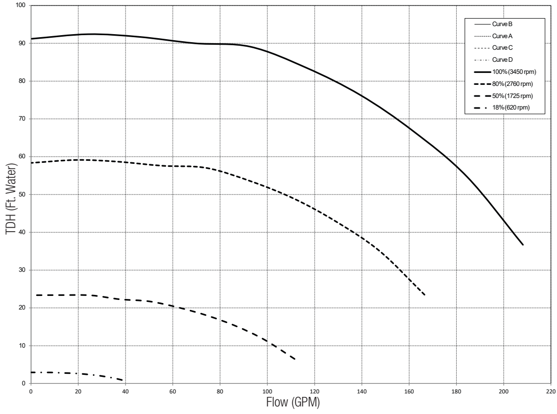
TriStar XL HCP3040VSP Performance Curves
