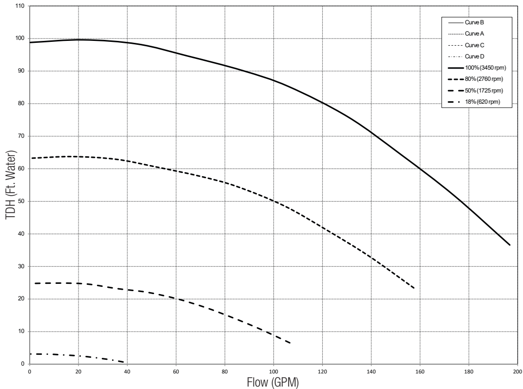
TriStar VSP32940 Performance Curves
