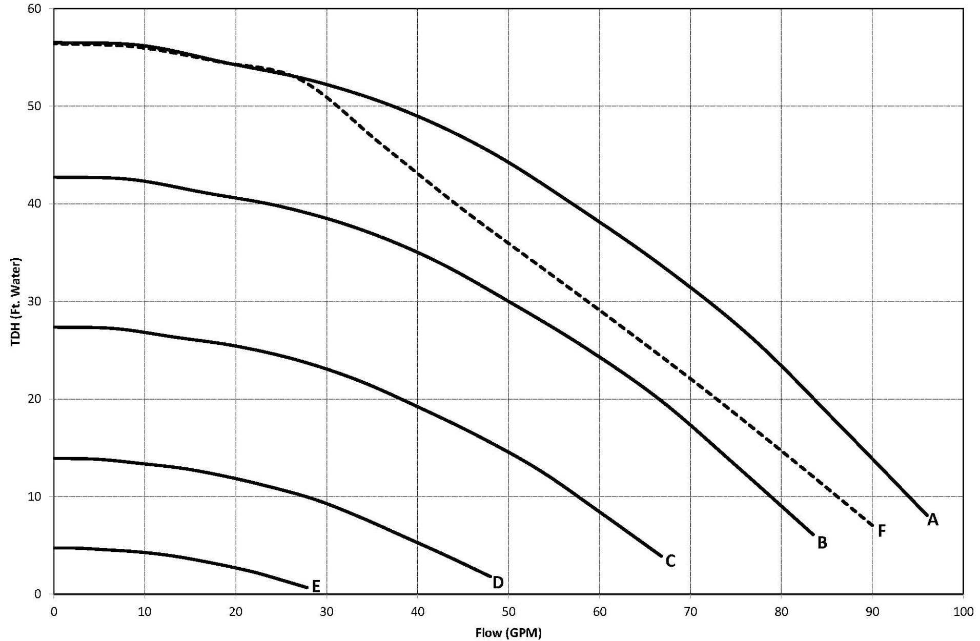
SP23520VSP Performance Curves
