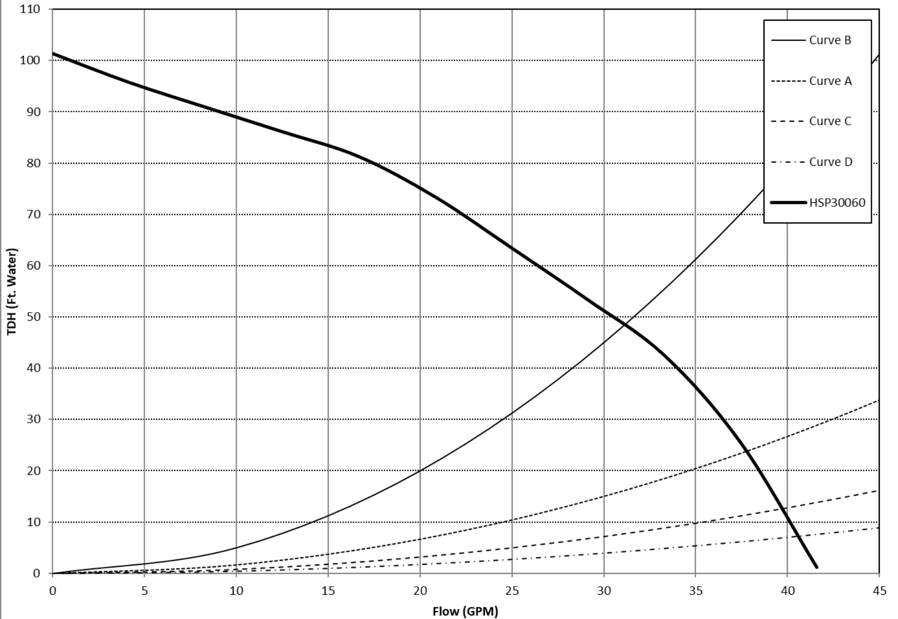
HSP30060 Performance Curve
