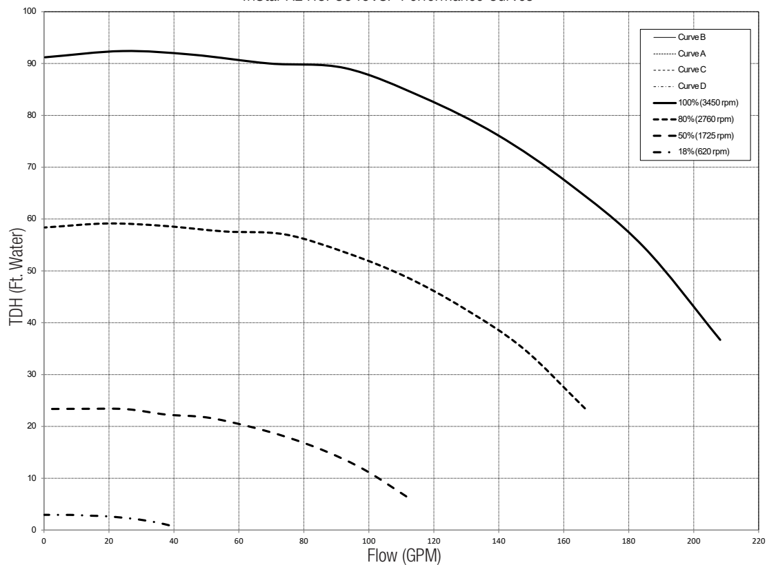
TriStar XL HCP3040VSP Performance Curves
