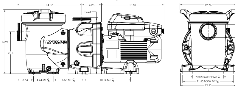
4.0 HP & 2.7 HP TRISTAR XL DIMENSIONS (INCHES)
